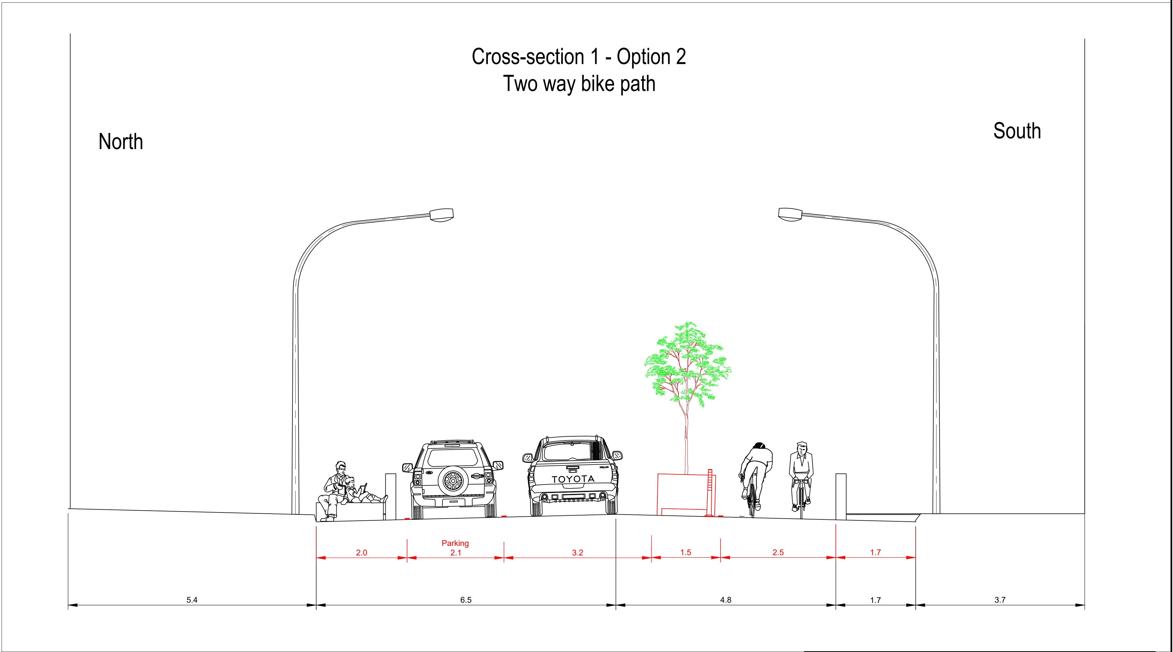
Cross-section 1:50
